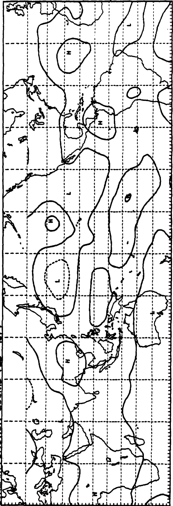
STREAM FUNCTION 200MB FEB 1974
